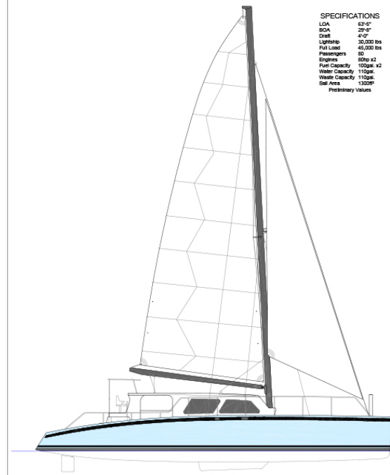
GC65 Outboard Profile
